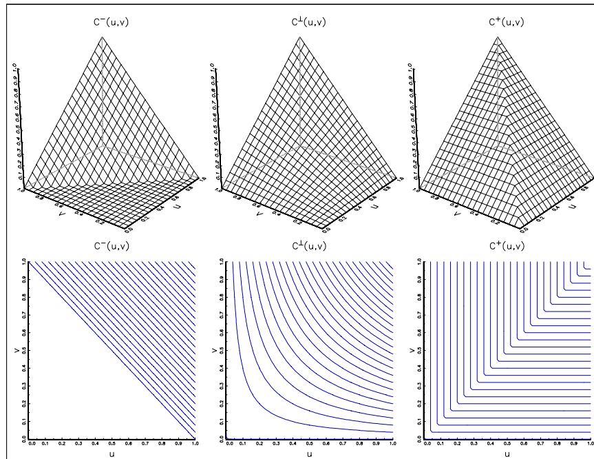
Figure 1: \mathbf{C}^- , \mathbf{C}^\perp and \mathbf{C}^+
