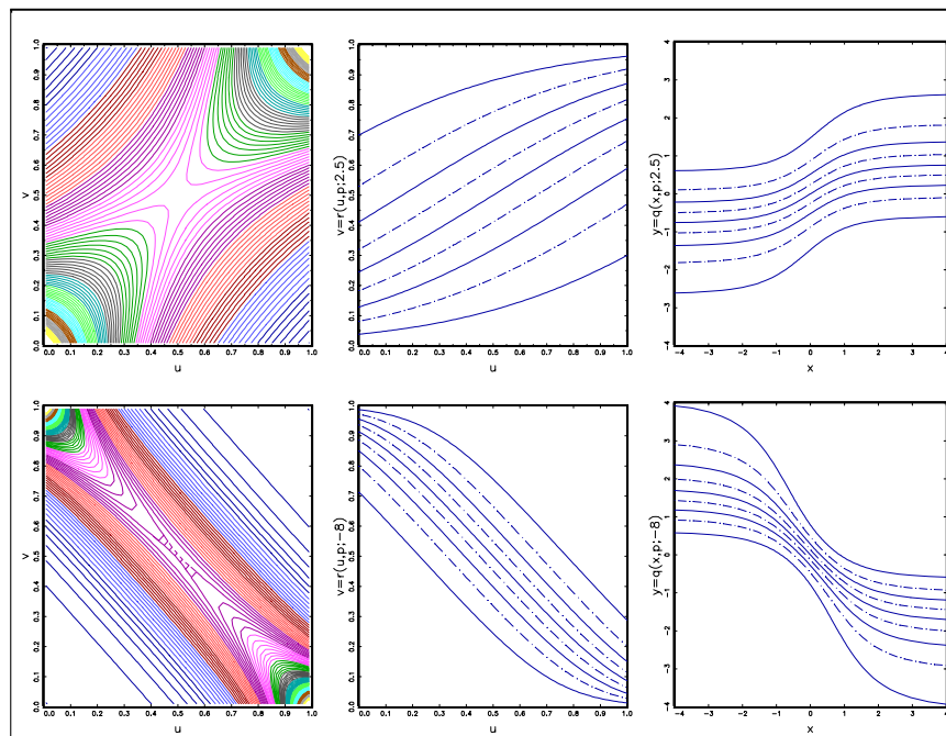
Figure 3: Frank copula densities, copula p^{th} quantile curves (for p = .1, .2, \dots, .9 ) for (u, v) and (x, y) under the hypothesis of Student margins ( \nu = 3 ) for \delta = 2.5 (upper plots) and \delta = -8 (lower plots)
