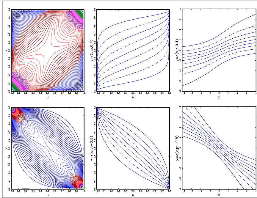
Figure 2: Gaussian copula densities, copula p^{th} quantile curves (for p = .1, .2, \dots, .9 ) for (u, v) and (x, y) under the hypothesis of Student margins ( \nu = 3 ) for \rho = 0.4 (upper plots) and \rho = -0.8 (lower plots)
